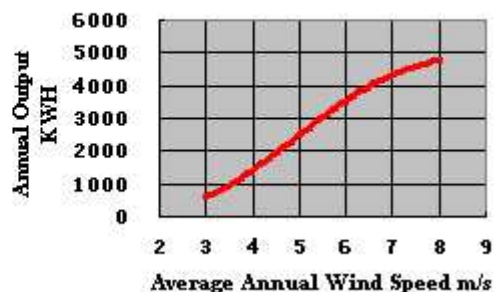
TAOS1500 Annual Output
