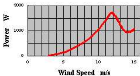
TAOS1500 Power Curve
